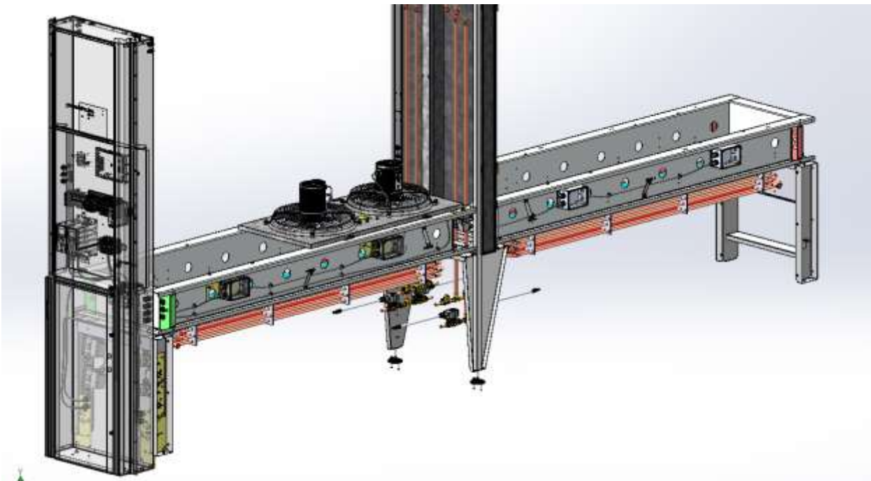
Figure 2: Double Depth Electric Heat Retrofit Kit
